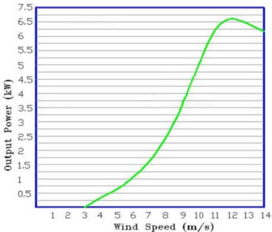
Output Power Curve API-5KW-FREE
