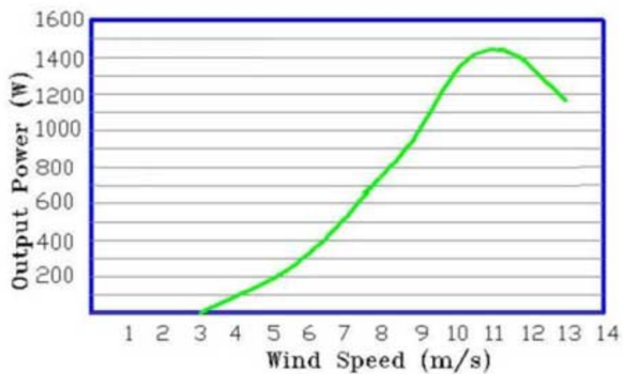
Output Power Curve - API-1KW-FREE
