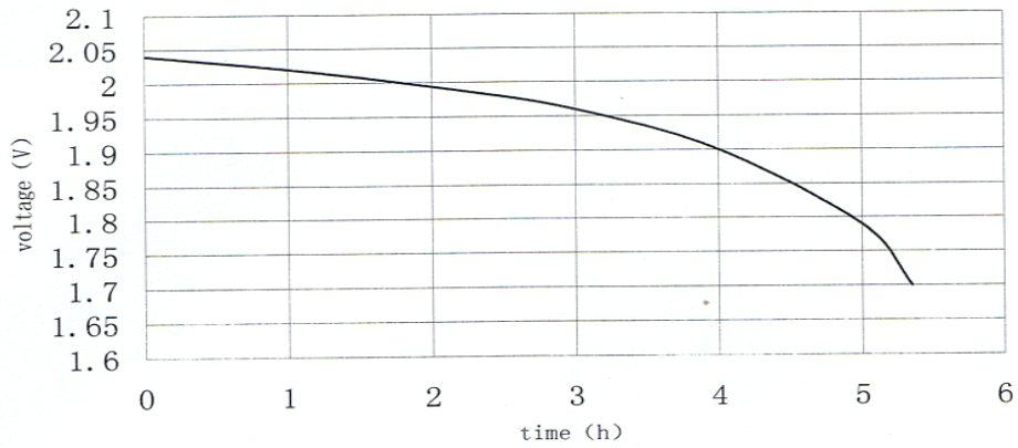
5hr discharge curve
